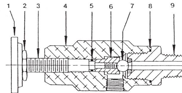
PART # 944-600
