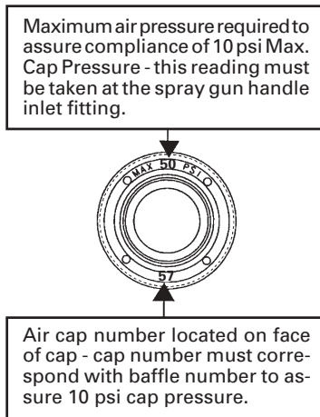
Figure 1 Baffle
