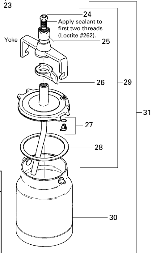
Figure 5 - Cup Drawing
